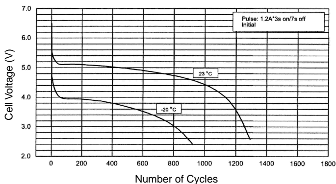
Pulse Discharge Characteristics of 2CR5
