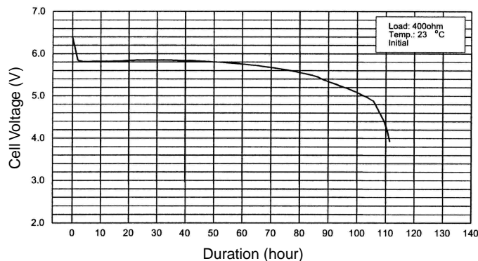
Discharge Characteristics of 2CR5
